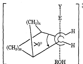
anti transition state (for trans addition)
